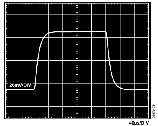
Figure 52. Small Signal Pulse Response, G = 1000 , R_L = 2\text{ k}\Omega , C_L = 100\text{ pF} , V_S = +5\text{ V} , V_{REF} = 2.5\text{ V}
