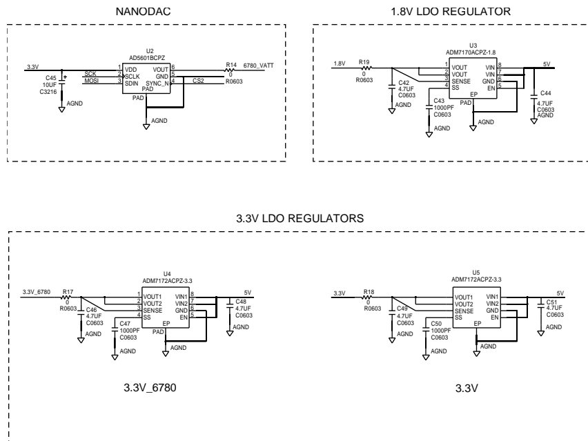
Figure 85. ADRF6780 Evaluation Board Schematic Page 3
