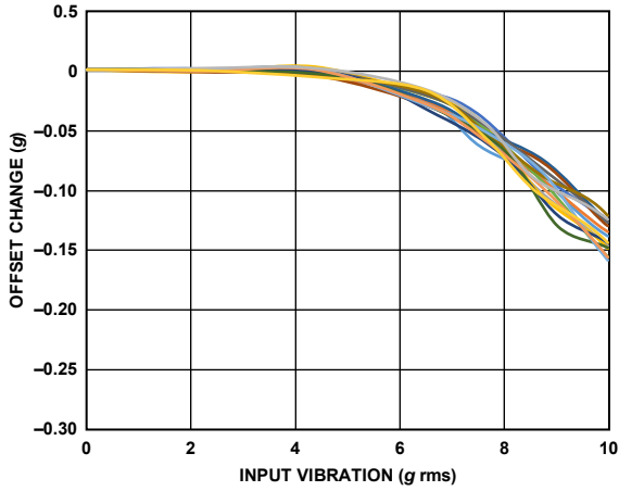
Figure 46. ADXL357 VRE, Z-Axis Offset from +1 g, ±10 g Range, Z-Axis Orientation = +1 g
