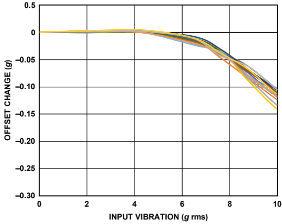
Figure 45. ADXL357 VRE, Y-Axis Offset from +1 g, ±10 g Range, Y-Axis Orientation = +1 g
