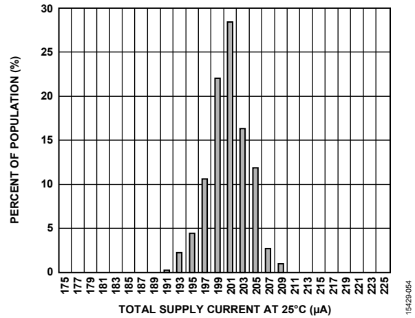
Figure 54. ADXL357 Total Supply Current, 3.3 V
