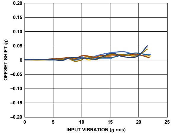
Figure 47. ADXL357 VRE, X-Axis Offset from -1 g, ±40 g Range, X-Axis Orientation = -1 g
