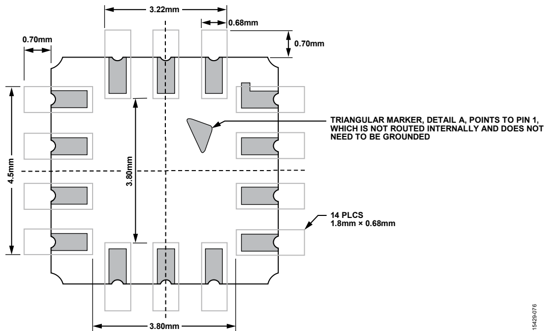
Figure 77. PCB Footprint Pattern and Dimensions in Millimeters
