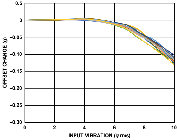
Figure 44. ADXL357 VRE, X-Axis Offset from +1 g, ±10 g Range, X-Axis Orientation = +1 g
