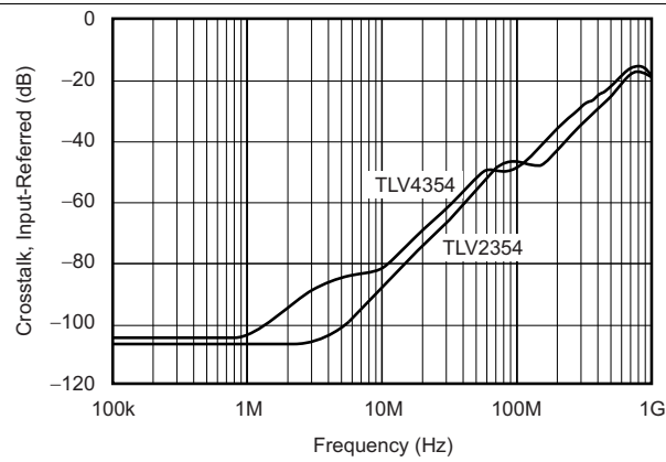
Figure 20. Channel-to-Channel Crosstalk
