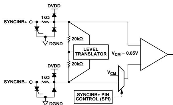
Figure 108. SYNCINB± Inputs
