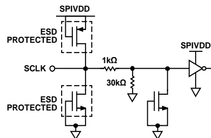
Figure 109. SCLK Input
