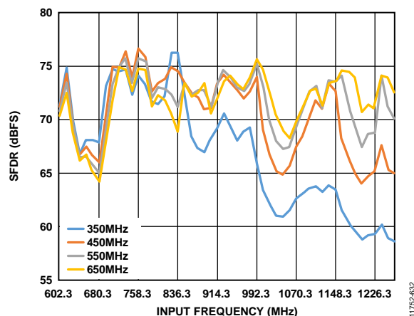
Figure 119. Buffer Current Sweeps, AD9680-1250 (SFDR vs. I_{BUFF} ); 600 \text{ MHz} < f_{IN} < 1300 MHz; Front-End Network Shown in Figure 115
