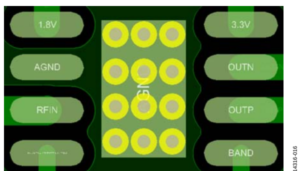
Figure 13. Evaluation Board Layout for the ADL5723 Package
