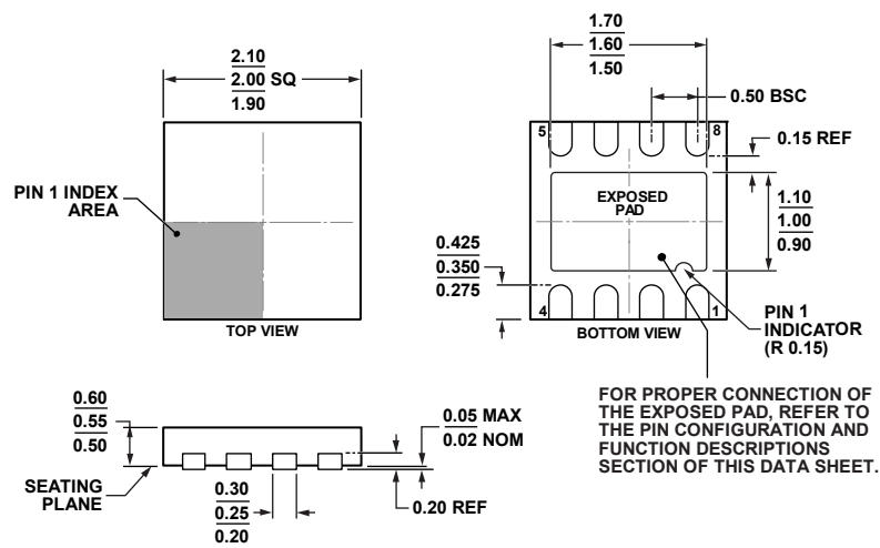
Figure 21. 8-Lead Lead Frame Chip Scale Package [LFCSP] 2.00 mm × 2.00 mm Body, and 0.55 mm Package Height (CP-8-10)
