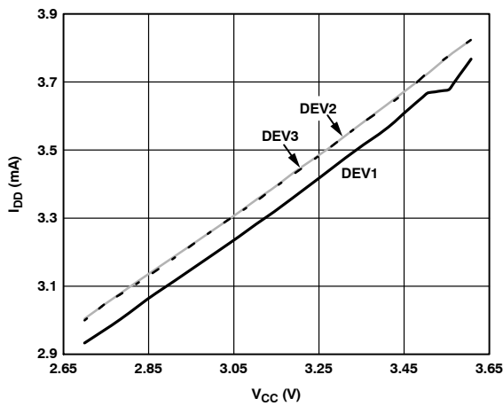
Figure 6. Supply Current vs. Voltage
