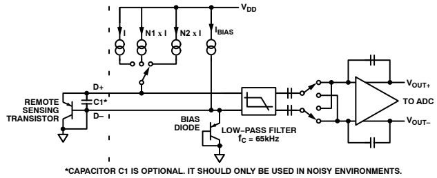
Figure 14. Signal Conditioning for Remote Diode Temperature Sensors
