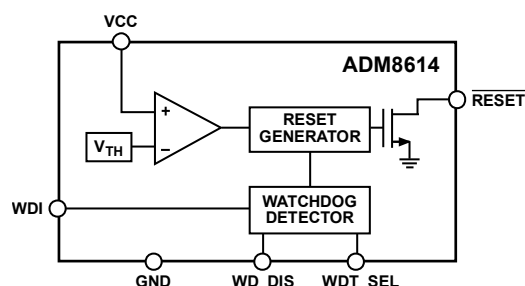
Figure 2. ADM8614 Functional Block Diagram
