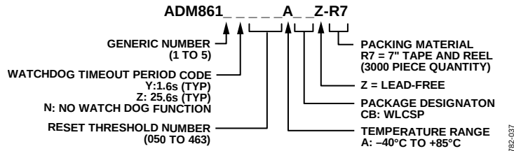
Figure 36. Ordering Code Structure
