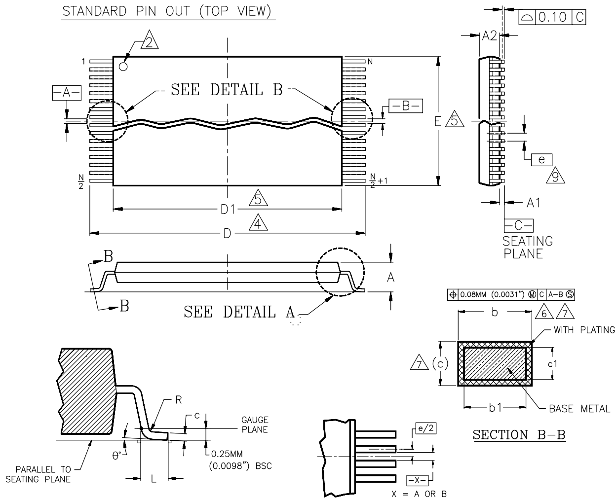
DETAIL A
