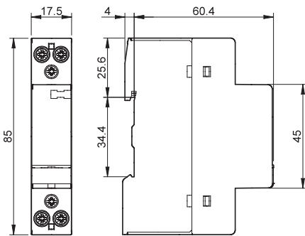
Type 22.72 Screw terminal
