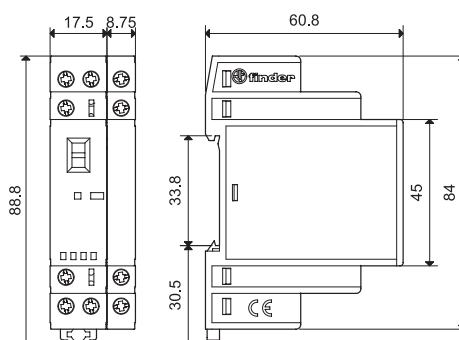
Types 22.32 + 022.33/022.35 Screw terminal
