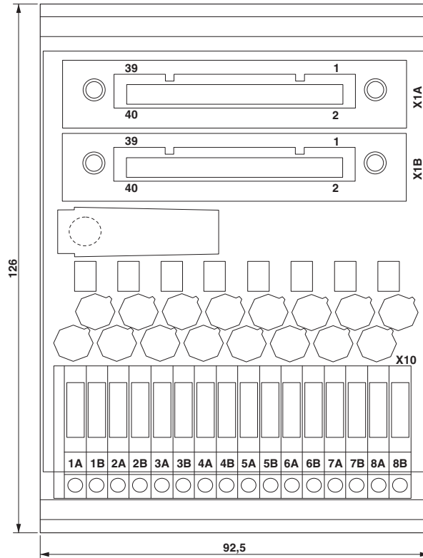
Dimensioned drawing
