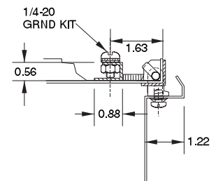
Hinge Detail (Section W-W)
