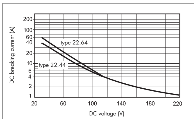
H 22 - Maximum DC1 breaking capacity - Type 22.44 / 22.64
