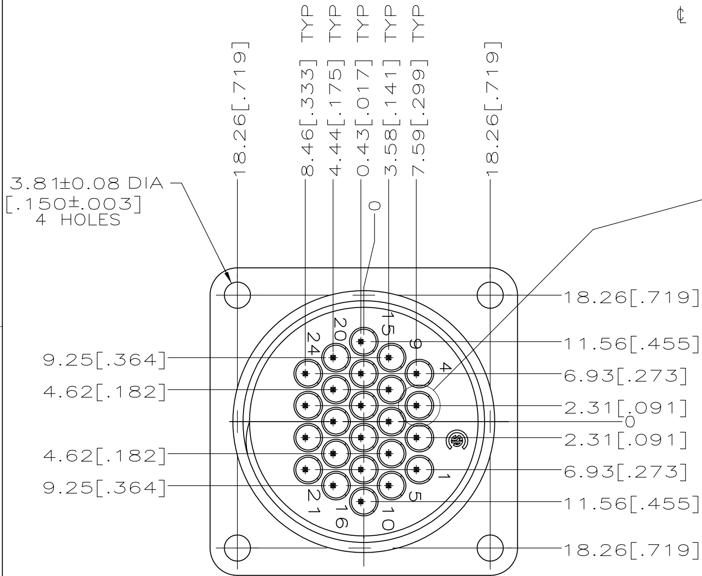
VIEW B-B
