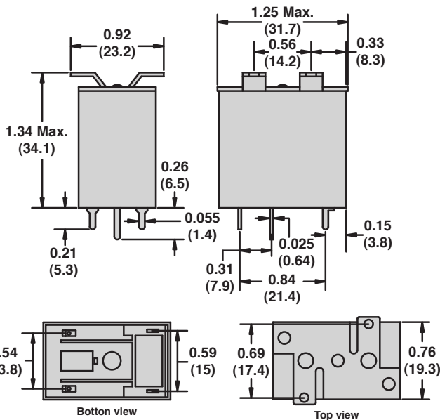
Top mounting bracket style (R1C4)
