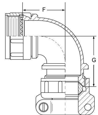
90° ENTRY ROTATABLE COUPLING 2M380MA137
