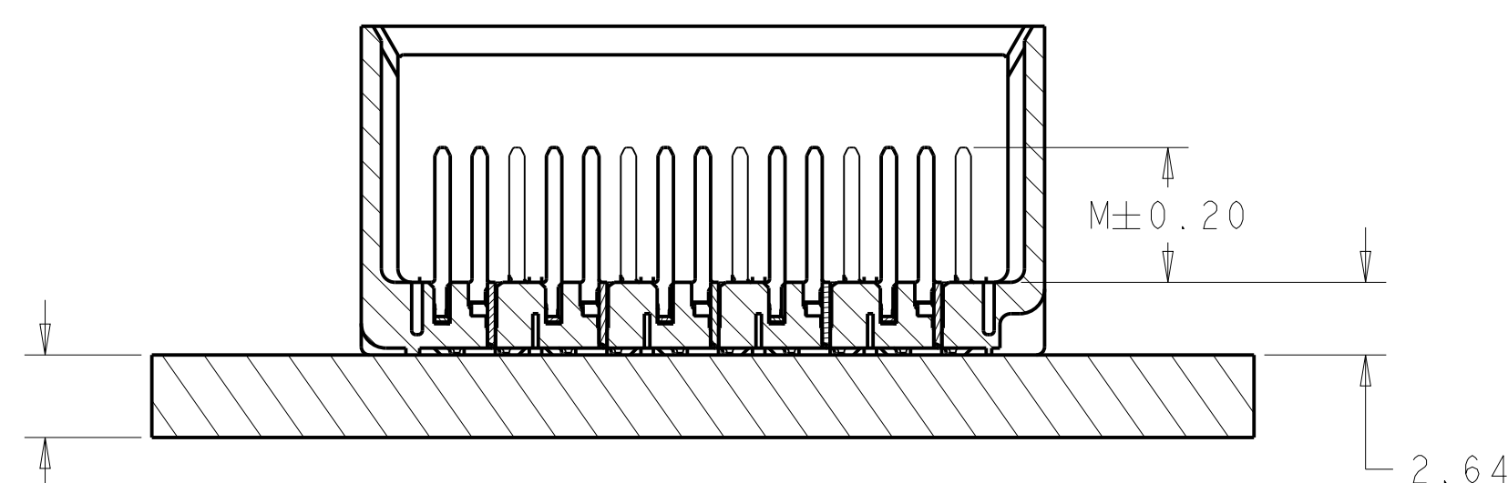
SECTION Z-Z
