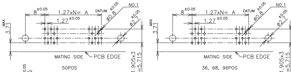
P.C. BOARD MOUNTING DIMENSIONS FIG.1
