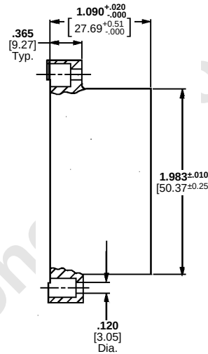
Plug Housing
