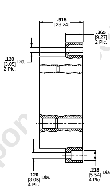
Receptacle Housing
