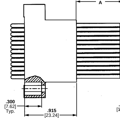
Plug Assembly
