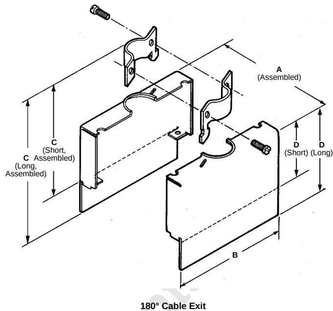
180° Cable Exit
