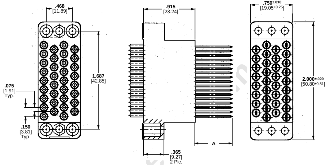
Plug Assembly
