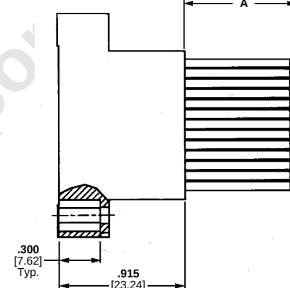
Receptacle Assembly
