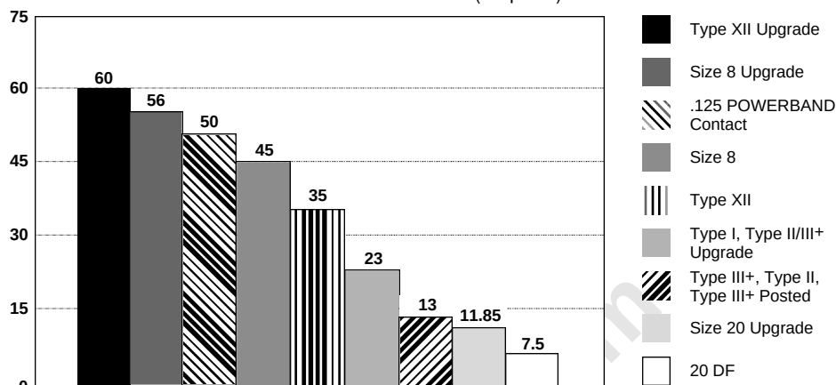
CONTACT CURRENT GUIDE Maximum Current (Amperes)
