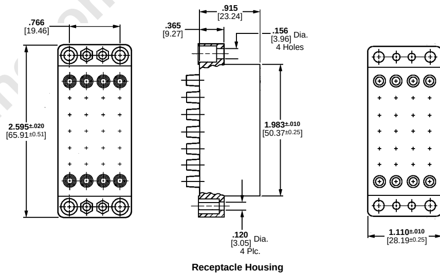
Receptacle Housing
