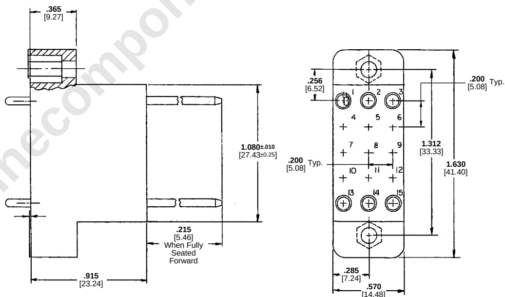
Plug Assembly (With Posted Pin Contacts)
