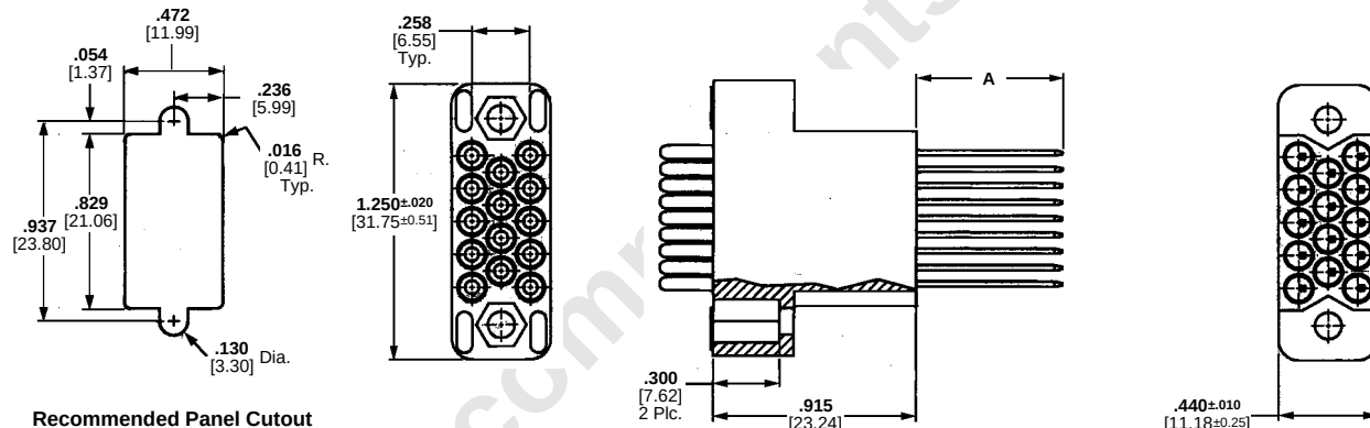
Plug Assembly
