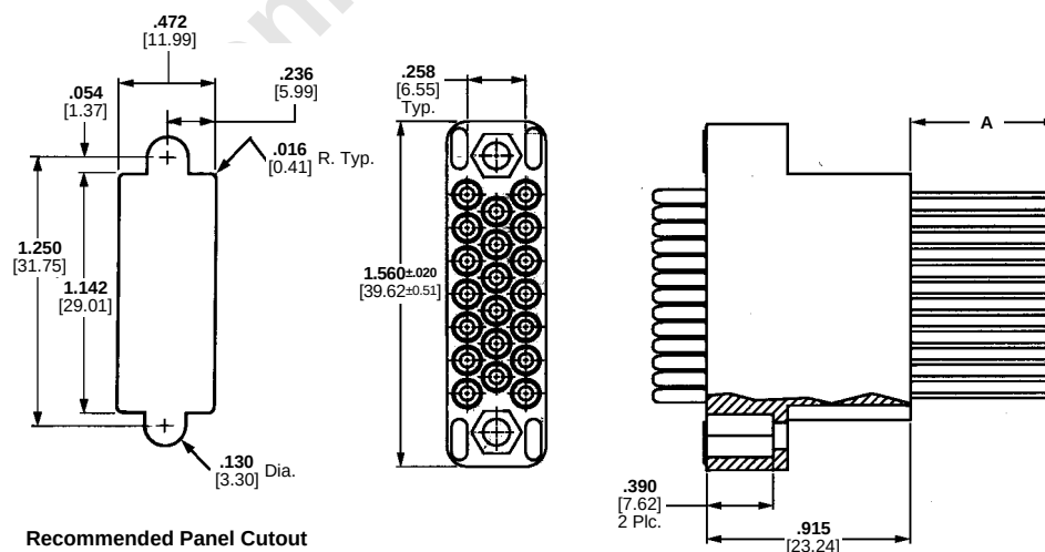
Plug Assembly
