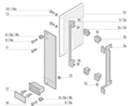
Item 8a, 3 U front panel mounting
