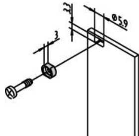
Front panel fixing
