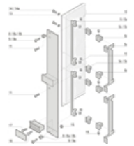
Item 8a, 6 U front panel mounting
