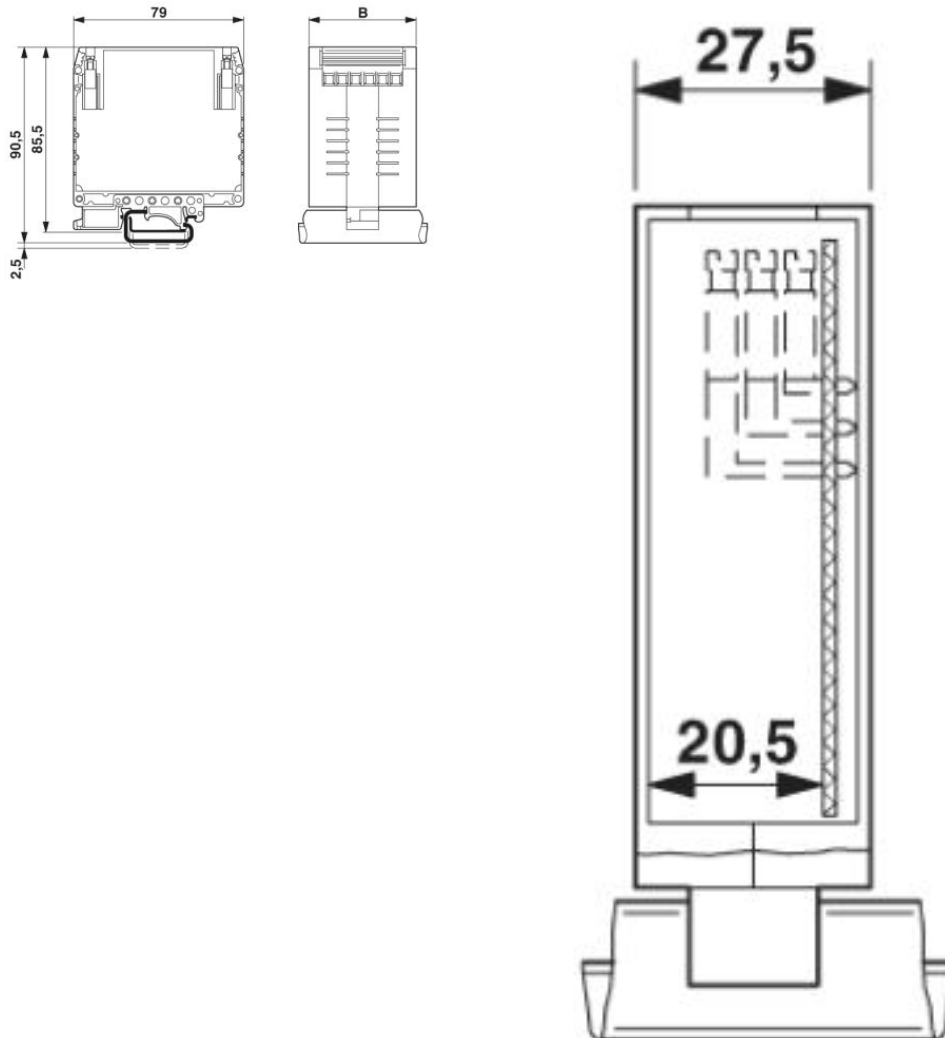
UEGM 25... und UEGM 27,5-SMD with 1 PCB, 6 positions or 12 positions (FS/FS)
