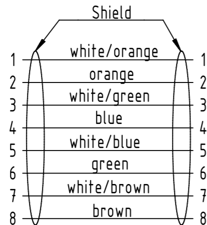
Loading-Plan acc. to TIA/EIA 568B
