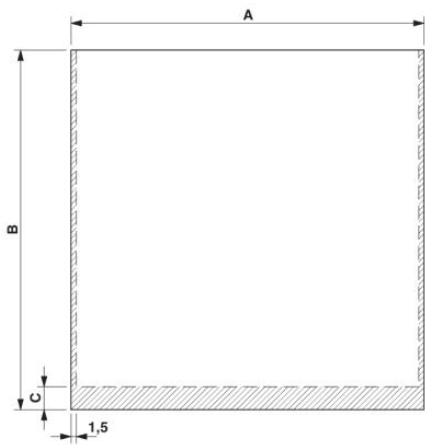
PCB 1, 7: Dimension A: 72.5 mm; B: 96.0 mm; C: 6.5 mm PCB 8, 13: Dimension A: 100.0 mm; B: 96.0 mm; C: 6.5 mm
