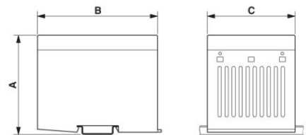
Dimension A=108 mm; dimension B=102 mm; dimension C=75 mm
