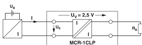
Application drawing
