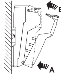
Figure 9-17 Snapping on a connector
