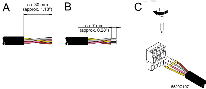
Figure 10-15 Assembling the motor circuit connector
