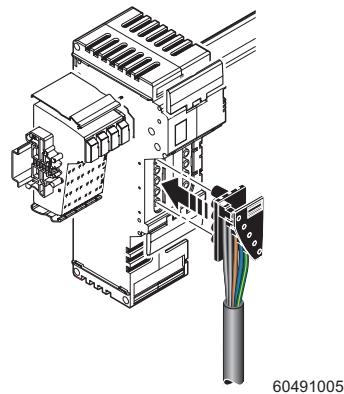
Figure 10-12 Connecting a power connector
