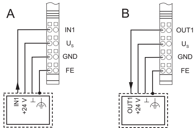
Figure 10-8 4-wire termination for digital devices
