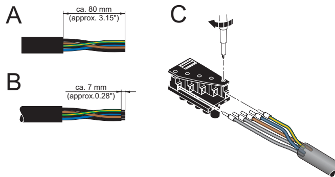
Figure 10-10 Assembling a power connector
