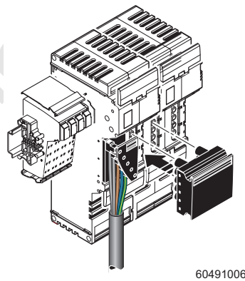
Figure 10-13 Inserting a power bridge
