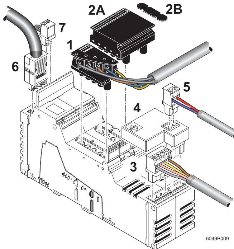
Figure 10-9 Power-level terminal with all possible connectors
