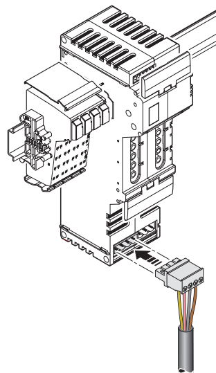
Figure 10-17 Inserting the motor circuit connector
