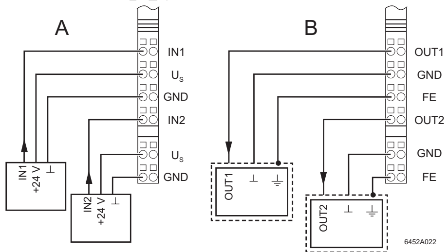
Figure 10-7 3-wire termination for digital devices
