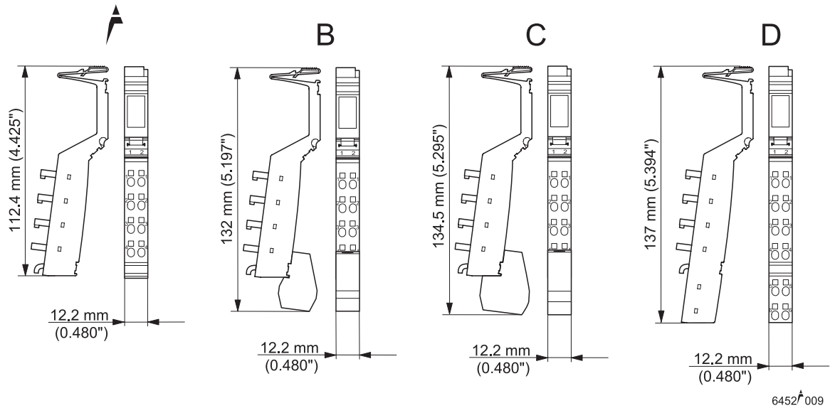
Figure 6-2 Connector dimensions
