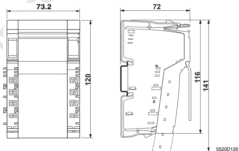
Figure 5-11 Dimensions of container housing 2 (in mm)
