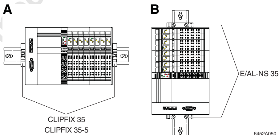
Figure 9-2 Mounting positions for an Inline station
