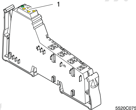
Figure 5-4 Function identification
