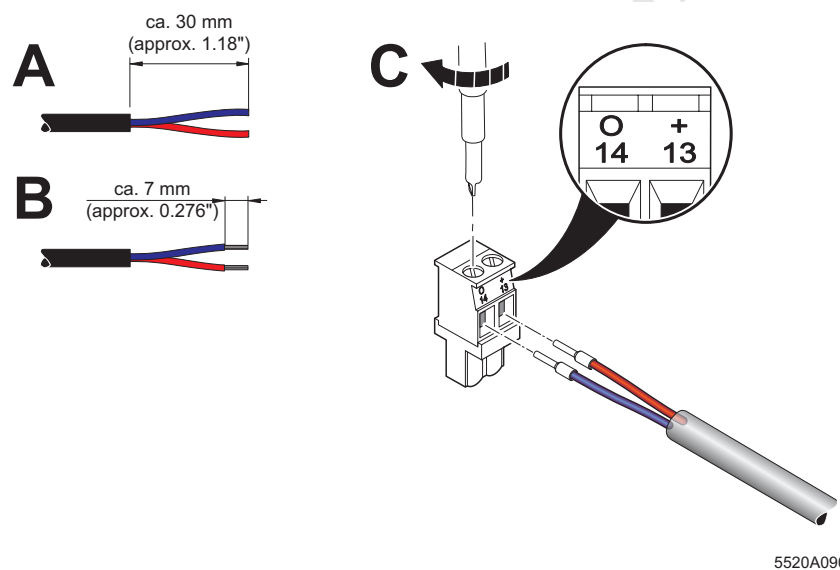
Figure 10-18 Assembling the connector for the brake
