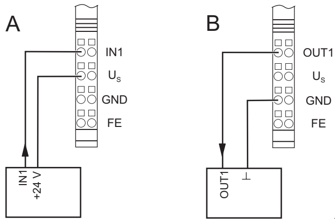
Figure 10-6 2-wire termination for digital devices
