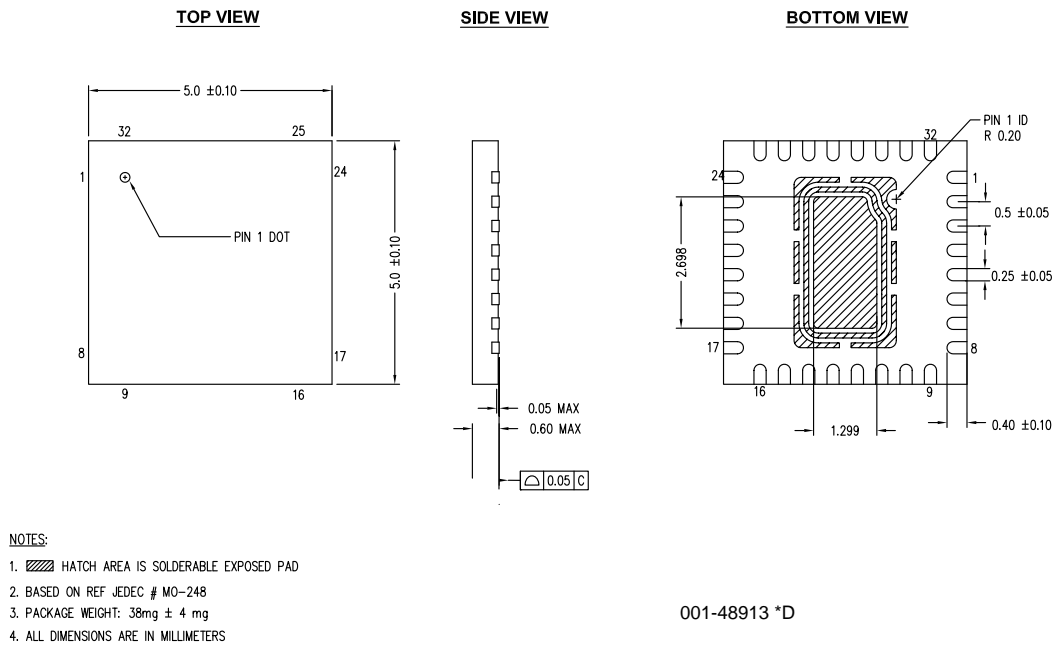
Figure 19. 32-pin QFN (5 × 5 × 0.55 mm) 1.3 × 2.7 E-Pad (Sawn Type) Package Outline
