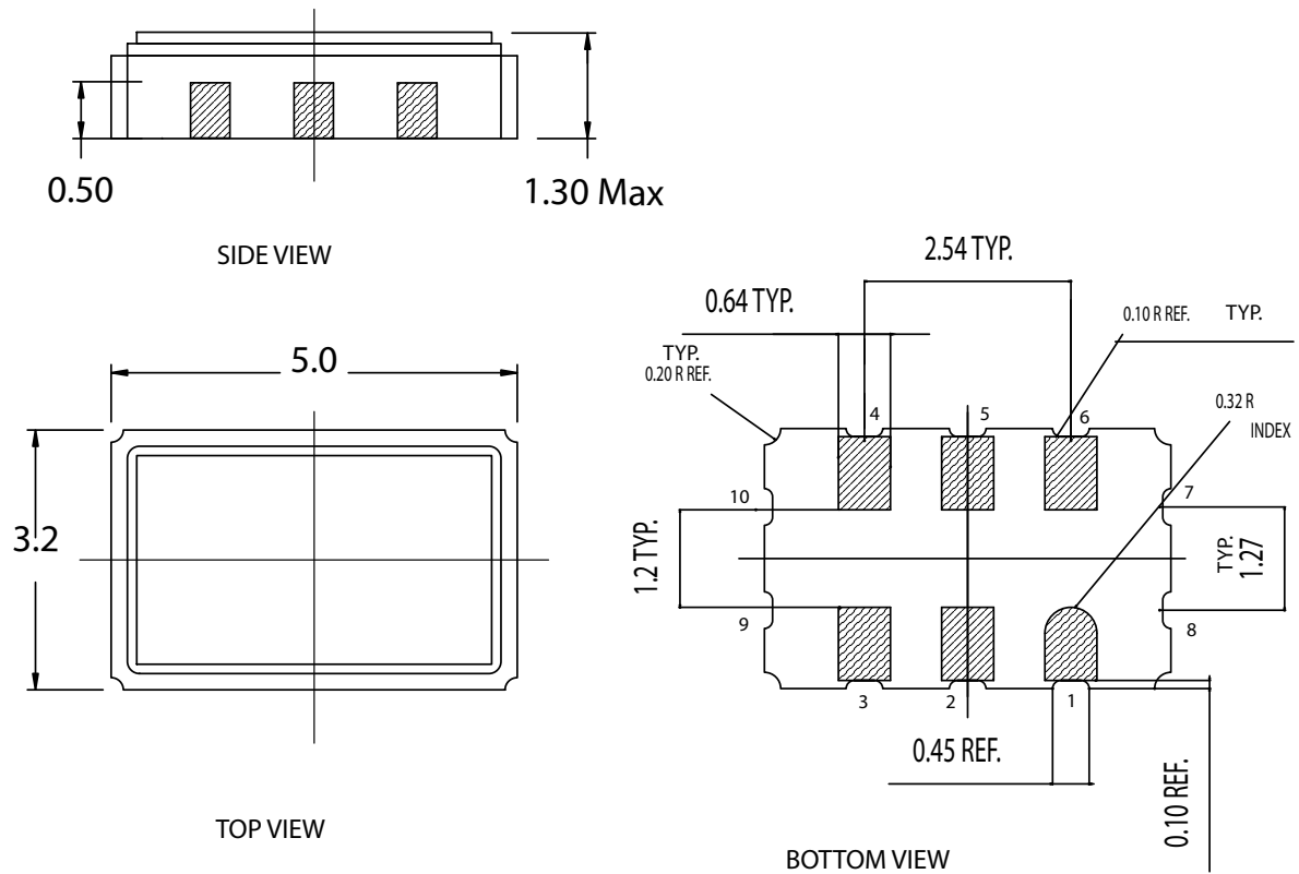
Figure 8. 6-Pin 3.2 × 5.0 mm Ceramic LCC LZ06A
