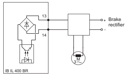
Connection diagram
