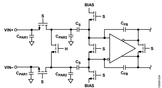
Figure 38. Switched-Capacitor Input
