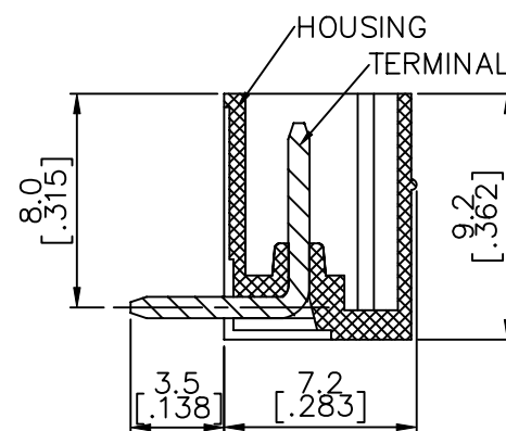
SECTION P-P
