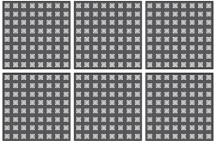
Tiled Matrices
