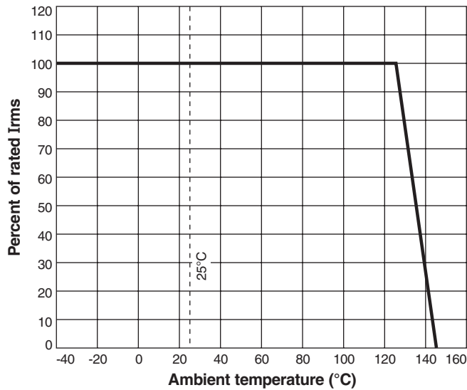
Irms Derating
