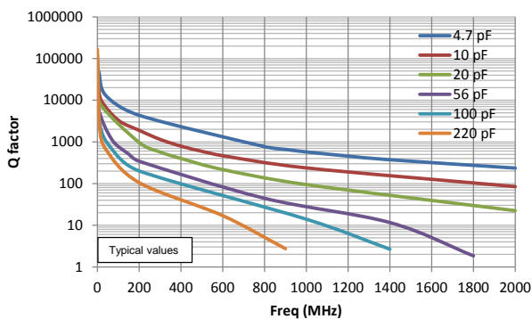
Q factor: 0805/R15S
