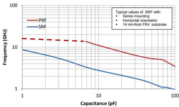
Resonant Frequency : 0201/R05L
