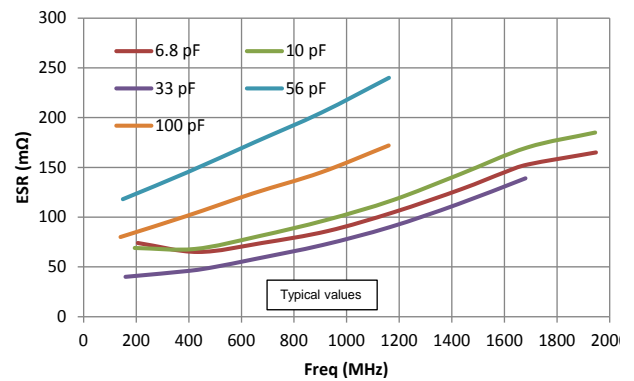
Equivalent Series Resistance: 0201/R05L
