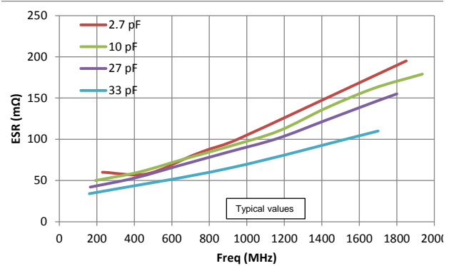
Equivalent Series Resistance: 0402/R07S
