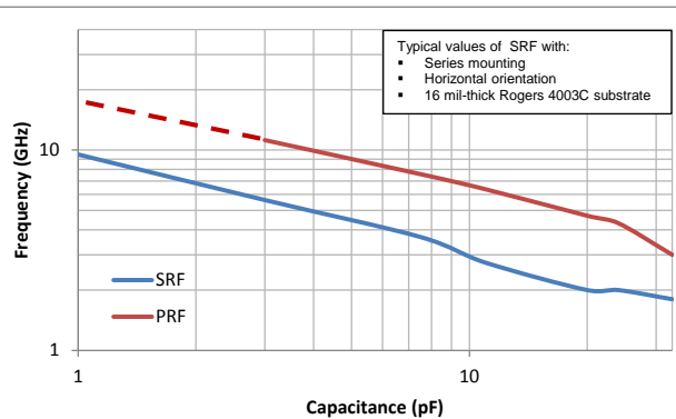
Resonant Frequency : 0402/R07S
