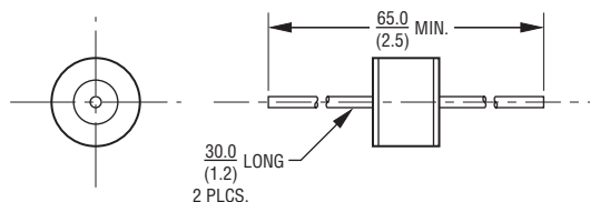
2027-XX-B10 — 0.8 mm (0.032 in.) dia. lead wire 2027-XX-C10 — 1.0 mm (0.040 in.) dia. lead wire (Not available in reelpack)
