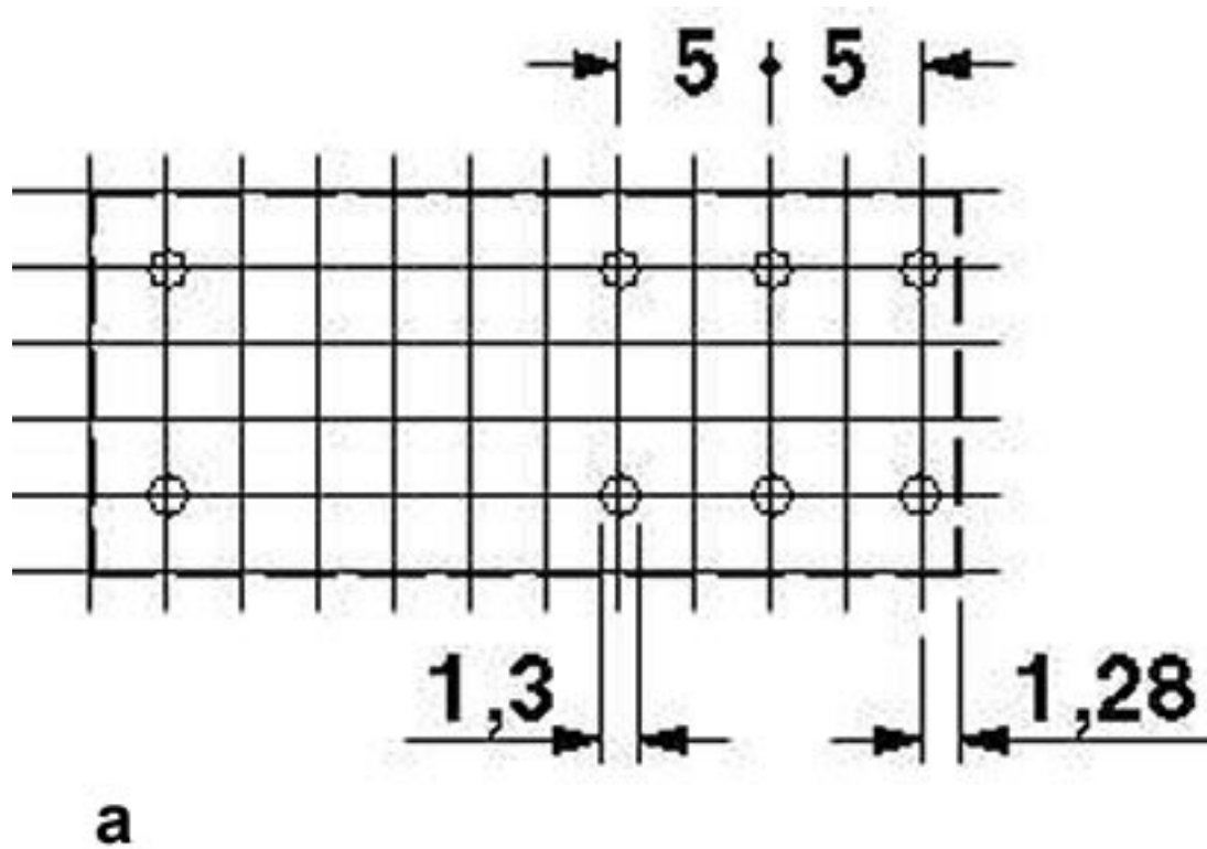
Drilling diagram
