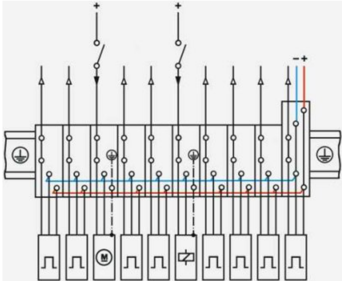
Circuit diagram
