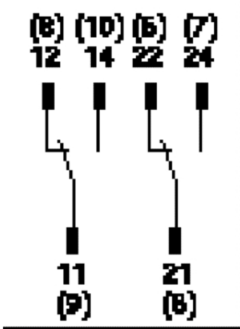
Circuit diagram
