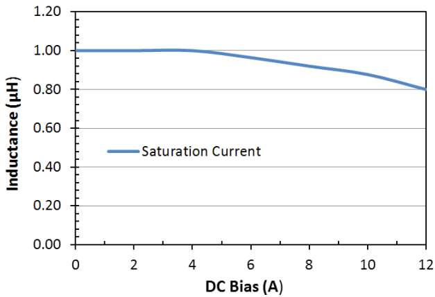
Saturation Current: LPM0530HI1R0ME
