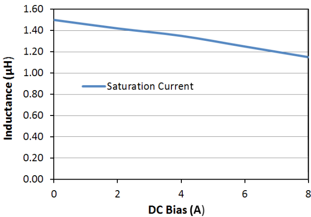
Saturation Current: LPM0520LR1R5ME
