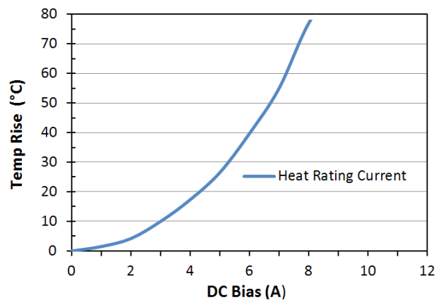
Heat Rating Current: LPM0630HI4R7ME
