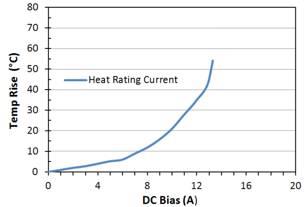
Heat Rating Current: LPM0630HI1R5ME
