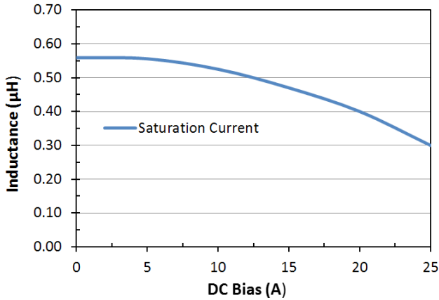
Saturation Current: LPM0630LRR68ME
