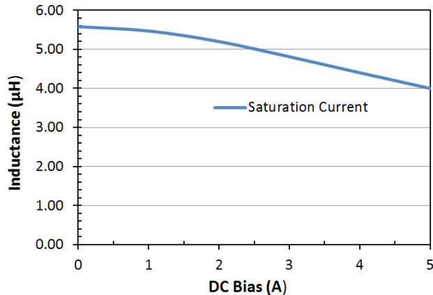
Saturation Current: LPM0520LR5R6ME
