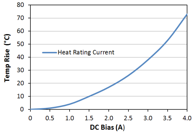
Heat Rating Current: LPM0630HI1R0ME
