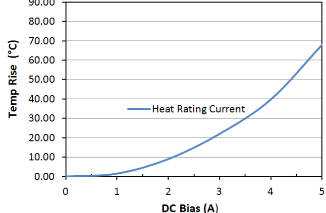
Heat Rating Current: LPM0520LR5R6ME
