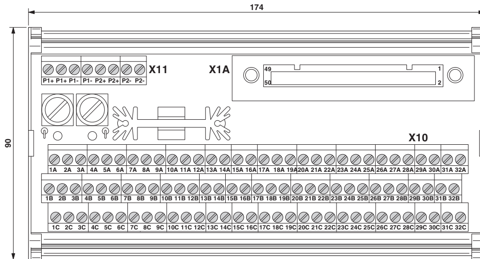
Dimensioned drawing
