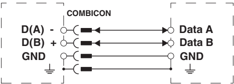
RS-485 connection
