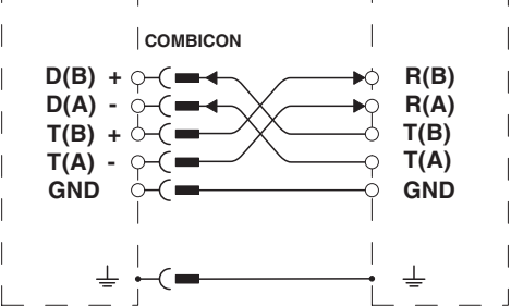
RS-422 connection
