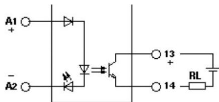
Circuit diagram
