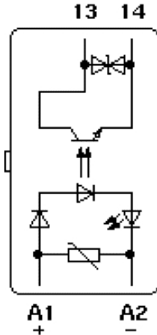
Circuit diagram
