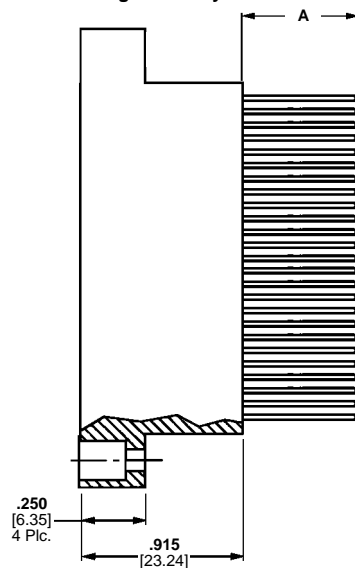
Receptacle Assembly
