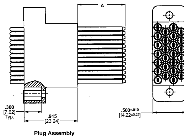
Plug Assembly
