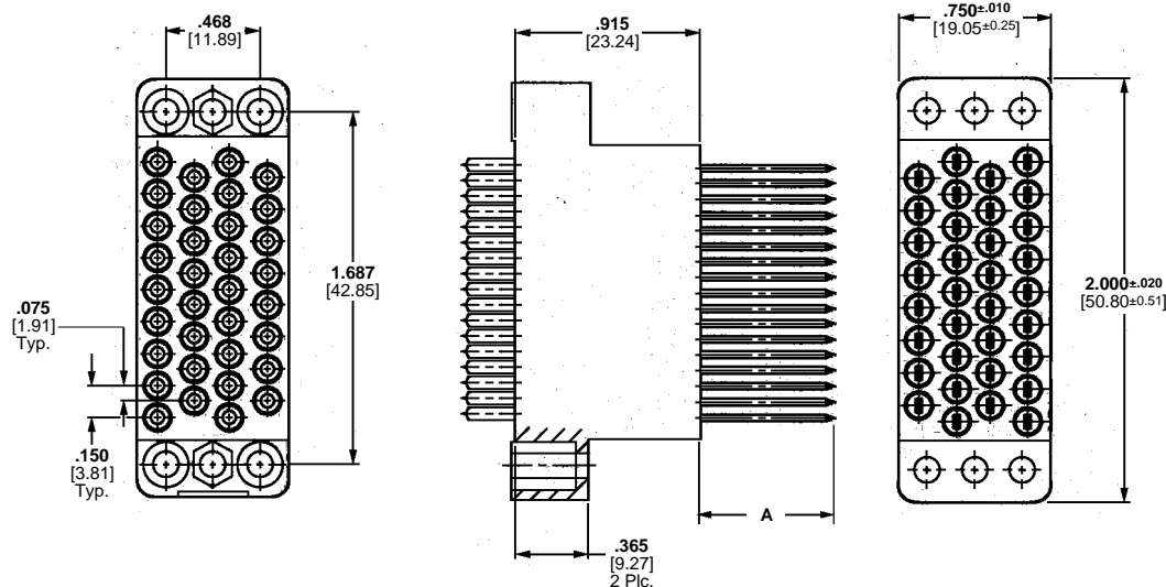
Plug Assembly
