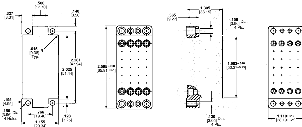
Plug Housing
