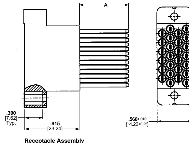
Receptacle Assembly
