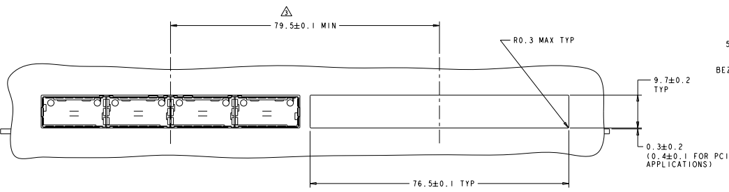
ONE SIDED CONFIGURATION SCALE 5:2
