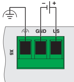
Connection diagram
