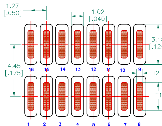
LAND PATTERNS FOR REFLOW SOLDERING
