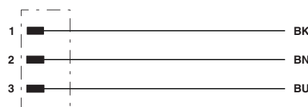
Contact assignment of 7/8" plug
