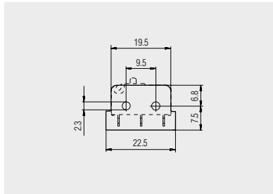
Insulating plate for solder terminal 0.5 mm: 231.005.021
