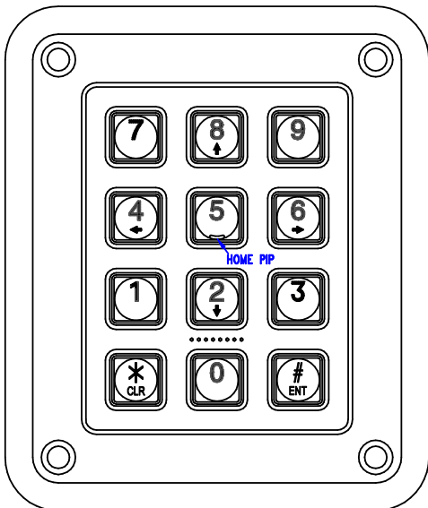
STD 12-WAY KEYPAD LAYOUT CALCULATOR
