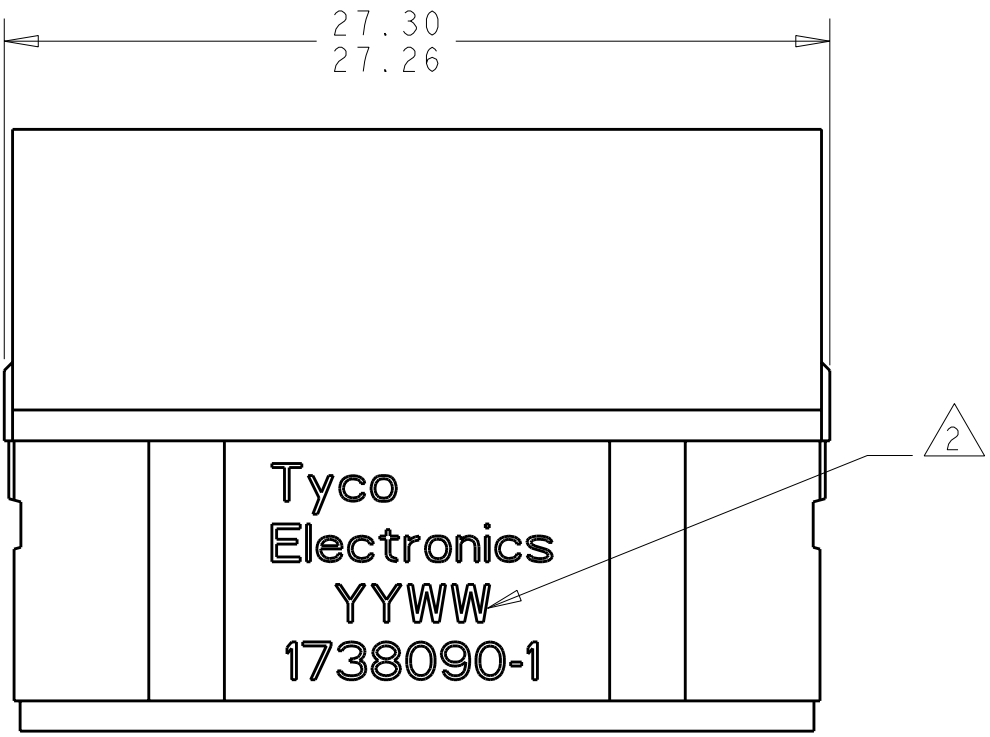
MATING FACE
